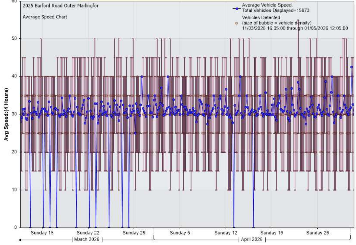
Average Vehicle Speed (MPH) vs. Time [2025 Barford Road Outer Marlingfor: Incoming]
