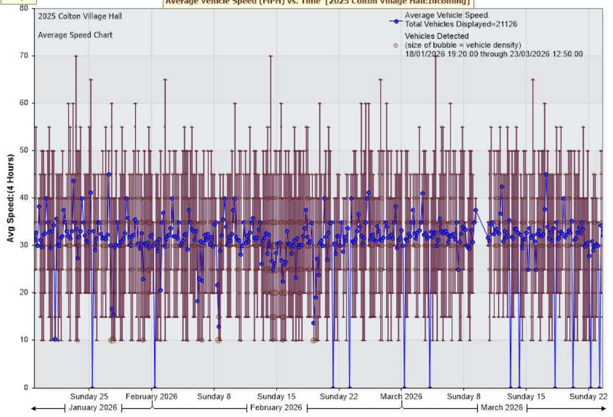
Average Vehicle Speed (MPH) vs. Time [2025 Colton Village Hall: Incoming]
